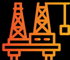
Petrochemicals
